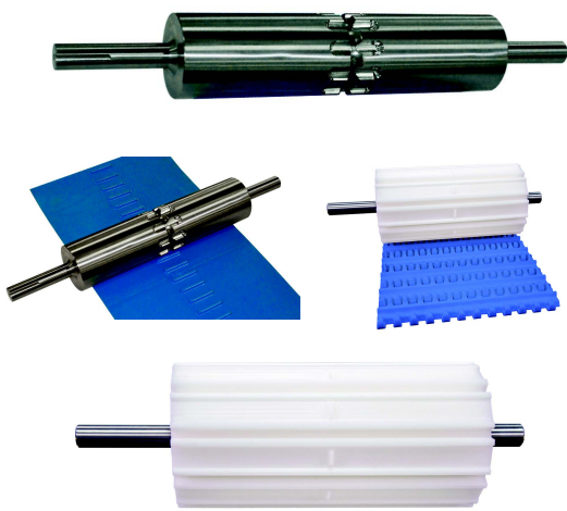
Sanitary Pulleys for Positive Drive and Plastic Modular Belts
